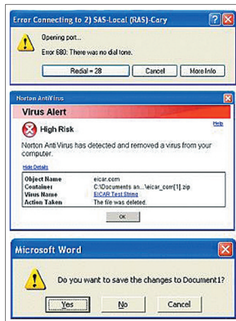
Figure 3. Can you spot the security message? (Part 2) Well-designed security messages have distinct visual and auditory properties that make them stand apart from all other message dialogs and indicate the criticality of the message.
