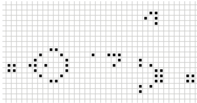
Figura 2.5: Glider gun
