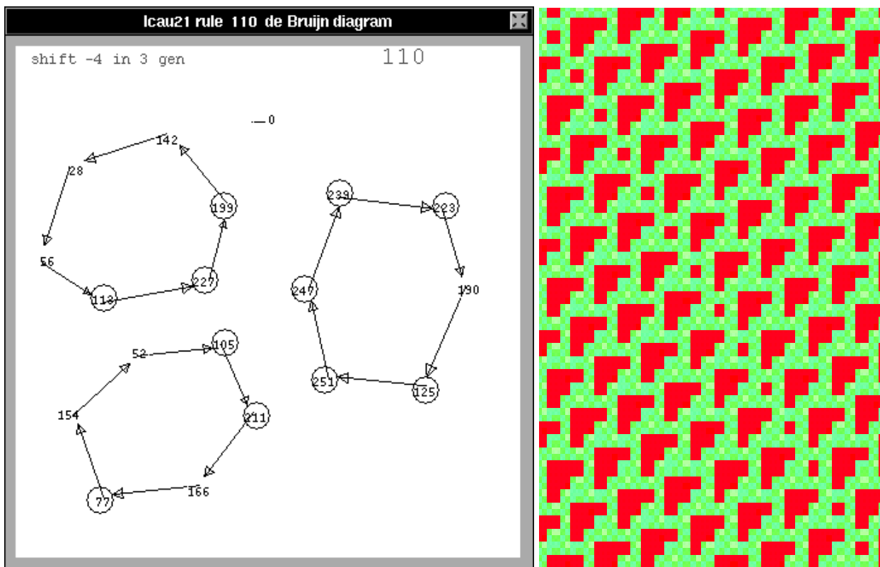
Figura 4.5: Glider A
